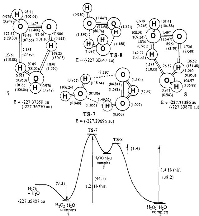
Figure 10. Hydrogen peroxide (7) and water oxide (8) hydrogen bonded to a mole of water and a comparison of the transition structures for a 1,2-hydrogen shift (TS-7) versus a 1,4-hydrogen shift (TS-8) for \text{H}_2\text{O}_2 hydrogen bonded to a \text{H}_2\text{O} molecule. (Optimized transition structures at the MP2/6-31G* level, HF/6-31G* geometry in parentheses; MP4SDTQ/6-31G*//MP2/6-31G* relative energies in kcal/mol (no ZPE), MP4SDTQ/6-31G*//HF/6-31G* values in parentheses.)
