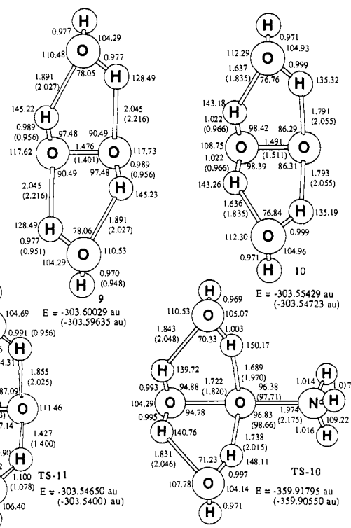
Figure 12. Optimized geometries for H 2 O 2 ( 9 ), H 2 OO ( 10 ), and the transition-state geometries for oxygen atom transfer from H 2 OO to NH 3 with two waters (TS-10) and the 1,4-hydrogen shift in H 2 O 2 hydrogen bonded to a second H 2 O (TS-11). (Optimized structures at the MP2/6-31G* level, HF/6-31G* geometry in parentheses; MP4SDTQ/6-31G**/MP2/6-31G* in kcal/mol (no ZPE), MP4SDTQ/6-31G**/HF/6-31G* values in parentheses.)
