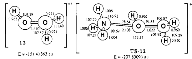
Figure 15. Byhydroxide cation (12) and its transition state for oxygen atom transfer with ammonia (TS-12). (Optimized geometries at HF/6-31G* level, energies at MP4/6-31G*.)
