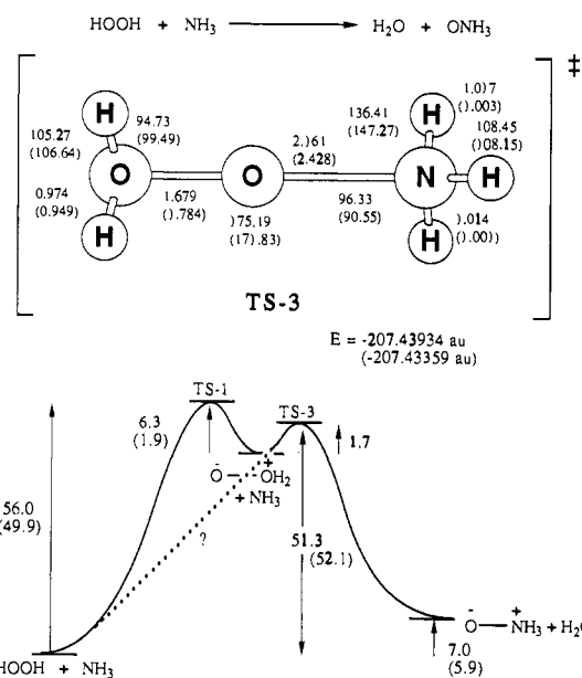
Figure 4. (a, top) Optimized transition structure at the MP2/6-31G* level (HF/6-31G* geometry in parentheses). (b, bottom) A comparison of the potential energy surfaces for 1,2-hydrogen shift (kcal/mol) in and oxygen atom transfer from hydrogen peroxide at the MP4SDTQ/6-31G* level (no ZPE) with use of the MP2 optimized geometry (MP4 energies at the HF geometries in parentheses).
