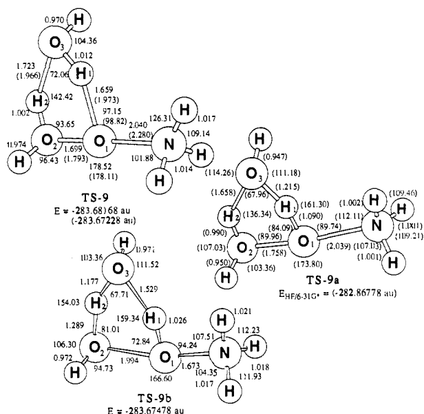
Figure 11. Transition structure (TS-9) for oxygen atom transfer from H 2 O to NH 3 with one water. (Optimized geometry at the MP2/6-31G* level, HF/6-31G* geometry in parentheses; MP4SDTQ/6-31G**/MP2/6-31G* relative energies in kcal/mol (no ZPE), MP4SDTQ/6-31G**/HF/6-31G* values in parentheses.) Optimized geometry (HF/6-31G* second-order saddle point) for oxygen atom transfer from H 2 O 2 to NH 3 with one water where the O 1 -H 1 bond is necessarily constrained (1.09 Å).
