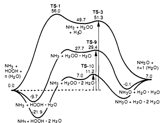
Figure 13. Activation barriers for oxygen atom transfer from H 2 O 2 to NH 3 catalyzed by zero, one, or two molecules of water (MP4SDTQ/6-31G**/MP2/6-31G* in kcal/mol without ZPE).
