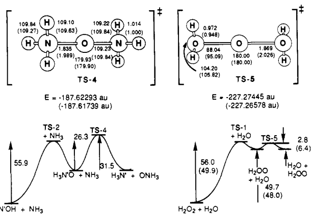
Figure 5. (a, left) 1,2-hydrogen shift (TS-2) versus oxygen atom transfer (TS-4) in hydroxylamine, (b, right) 1,2-hydrogen shift (TS-1) versus oxygen atom transfer (TS-5) in hydrogen peroxide (optimized transition structures at the MP2/6-31G* level, HF/6-31G* geometry in parentheses; MP4SDTQ/6-31G*/MP2/6-31G* relative energies in kcal/mol (no ZPE), MP4SDTQ/6-31G*/HF/6-31G* values in parentheses).
