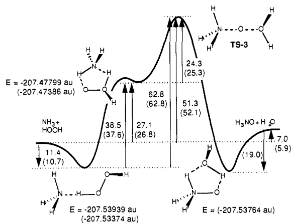
Figure 8. The potential energy profile for oxygen atom transfer from \text{H}_2\text{O}_2 to \text{NH}_3 at the MP4SDTQ/6-31G**/MP2/6-31G* level in kcal/mol; MP4 energies with use of the HF optimized geometries in parentheses.
